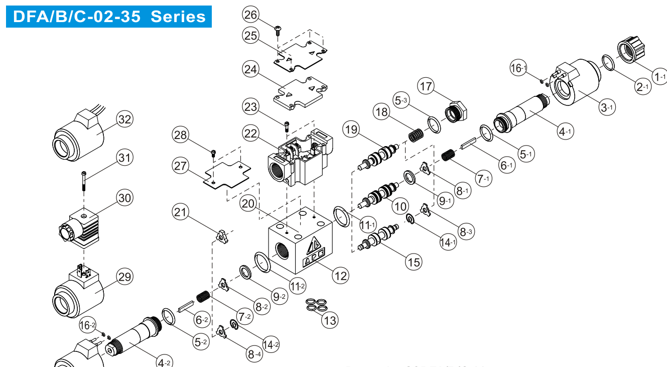
Parts List Of DFA/B/C-02
